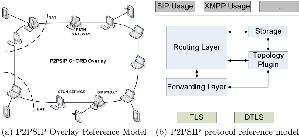
Fig. 2. P2PSIP reference models
