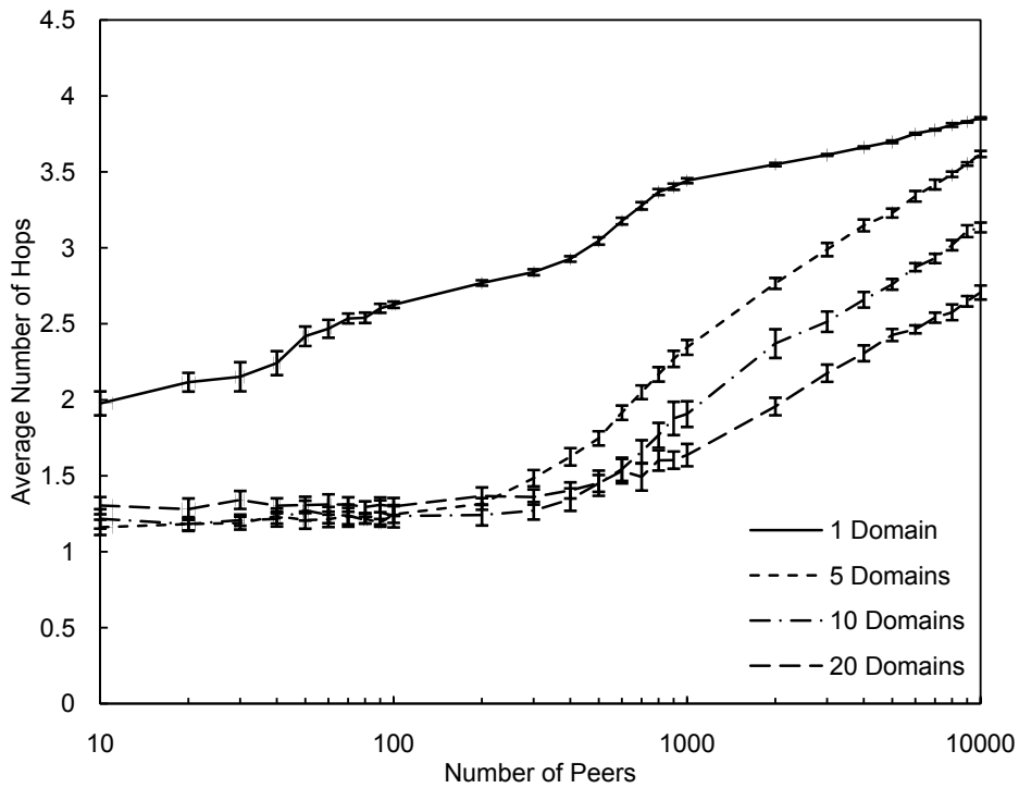
Fig. 10. Domain Routing Performance for Value Lookups
