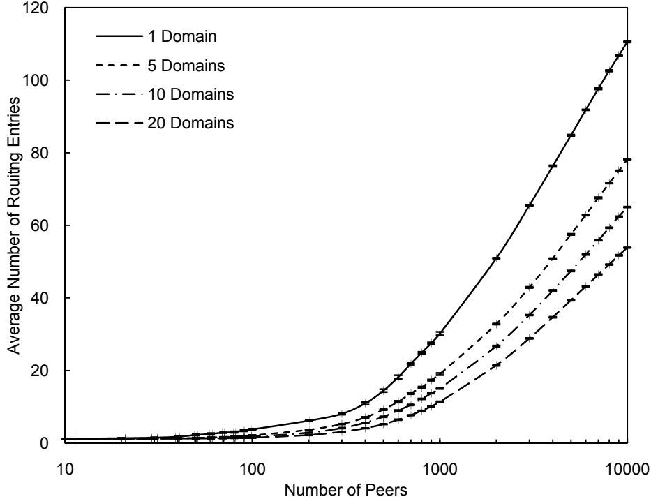
Fig. 12. Average number of entries in peers routing tables
