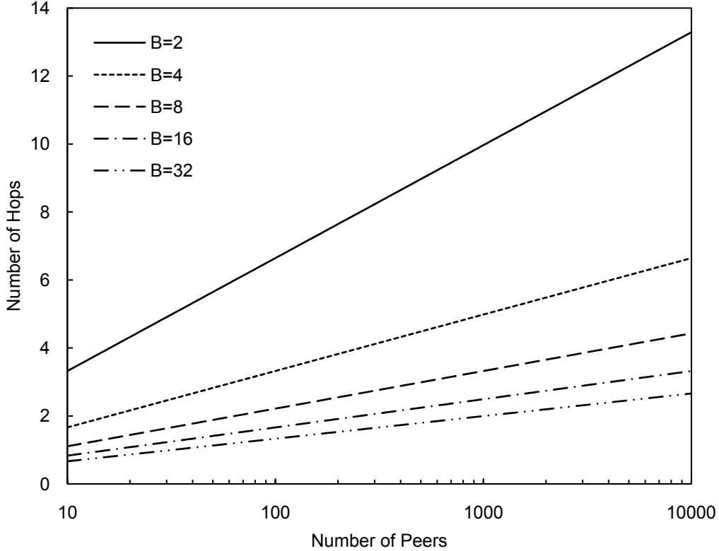
Fig. 7. Routing Performance
