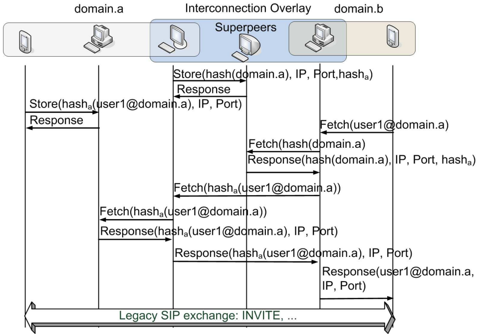
Fig. 5. H-P2PSIP Signalling
