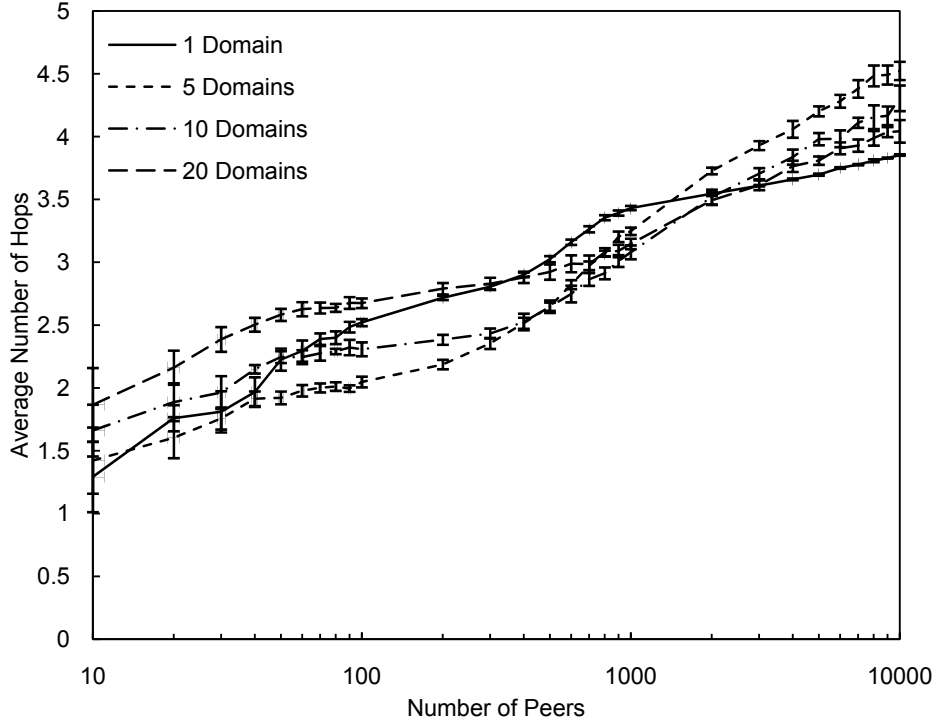
Fig. 8. Global Routing Performance for Value Lookups
