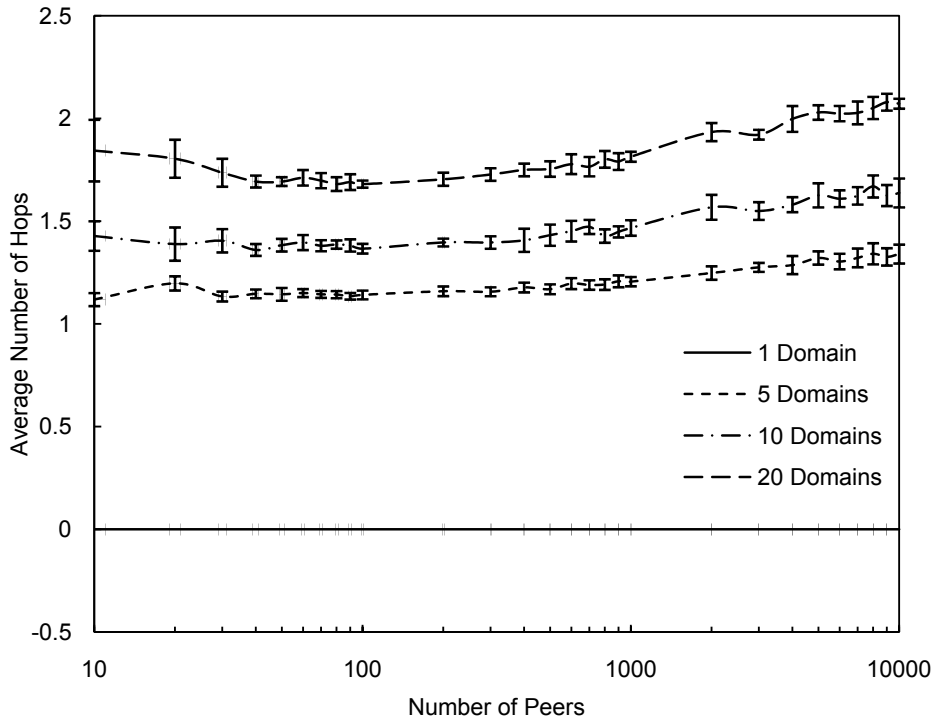
Fig. 9. Interconnection Overlay Routing Performance for Value Lookups
