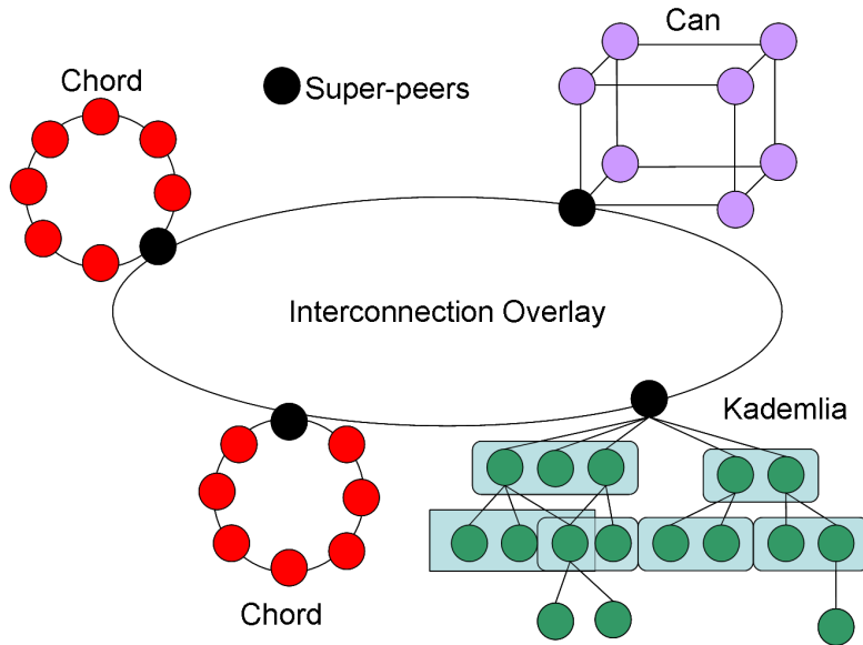
Fig. 1. Hierarchical Overlay Architecture
