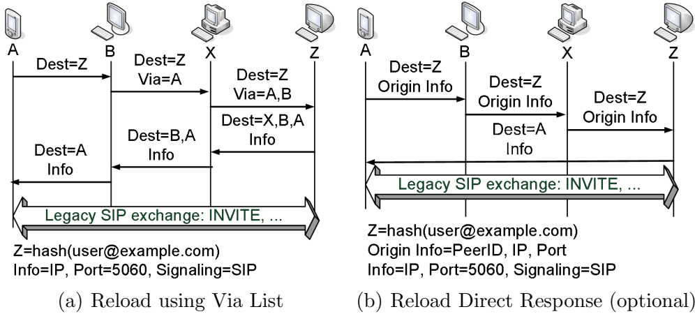
Fig. 3. Different Request-Response Models
