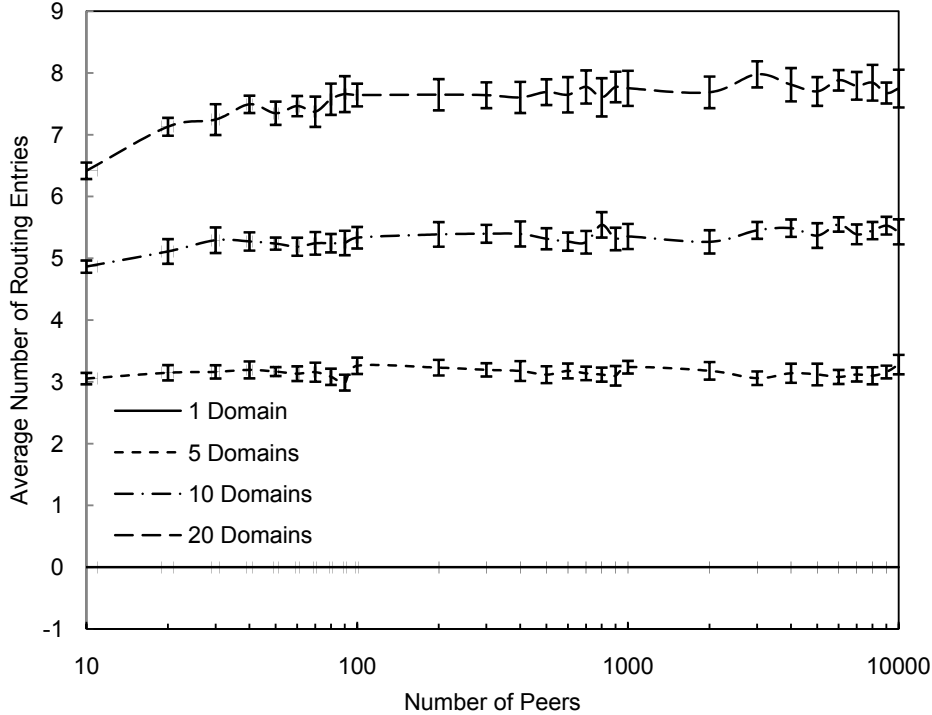
Fig. 11. Average number of entries in Interconnection Overlay routing tables
